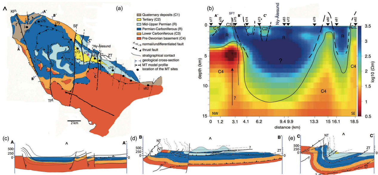
Figure 5. The preferred 2D MT model displayed together with bedrock geology for comparison. (a) A simplified surface geology map for Brøggerhalvøya illustrating the major fold–thrust belt structures and younger, crosscutting normal fault systems; simplified and redrawn from Bergh et al. (2000). (b) The 2D MT model. The MT model anomalies (R, C1 – C4) reasonably correspond with the geology and their interpretation is listed in the colour key in a coinciding manner with the bedrock map. Geological cross-sections that are redrawn from Bergh et al. (2000) are displayed in (c) through (e).
