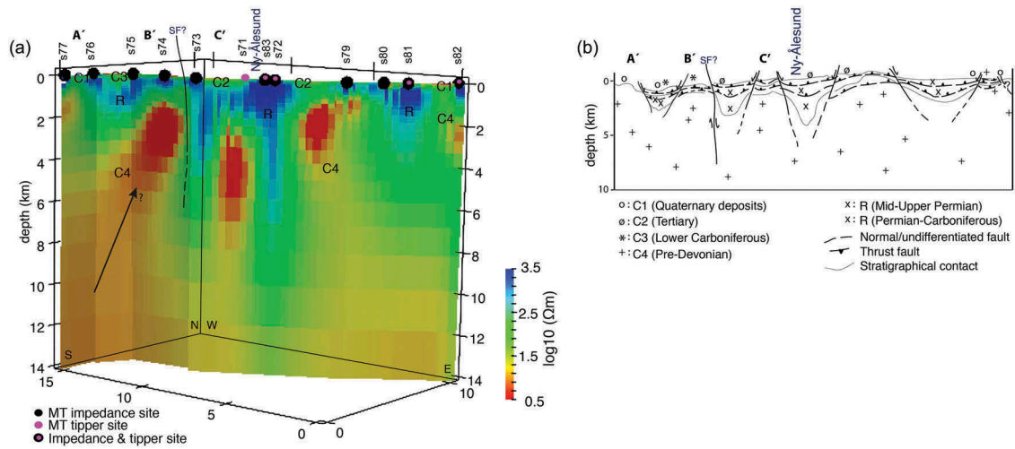
Figure 7. (a) The preferred final 3D model obtained by inverting the full impedance tensor by including detailed bathymetry and the tipper data. The 3D model is supported by the 2D result presented earlier and reflects a geologically meaningful reconstruction of the subsurface bedrock architecture. Interpretation of the model anomalies (R, C1 – C4) can be read from the colour key in Fig. 5. (b) Schematic presentation of the MT final model's geological and structural interpretation along the studied WNW-ESE profile, showing a horst-graben geometry of alternating, uplifted pre-Devonian unit (C4) and down-faulted Permian-Carboniferous strata (C2 – C3, R).
