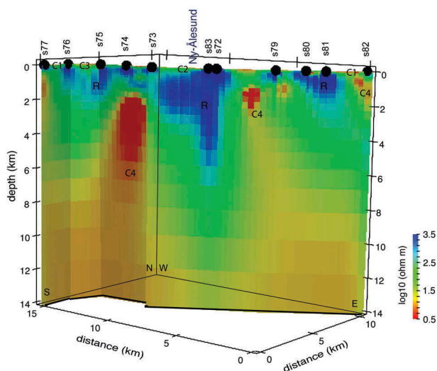
Figure 6. The 3D resistivity model obtained by inverting all the four components of the impedance tensor. The model has an overall misfit RMS 1.68, obtained after 300 iterations. Data fits of the model are displayed site by site with black solid lines in Fig. 8.
