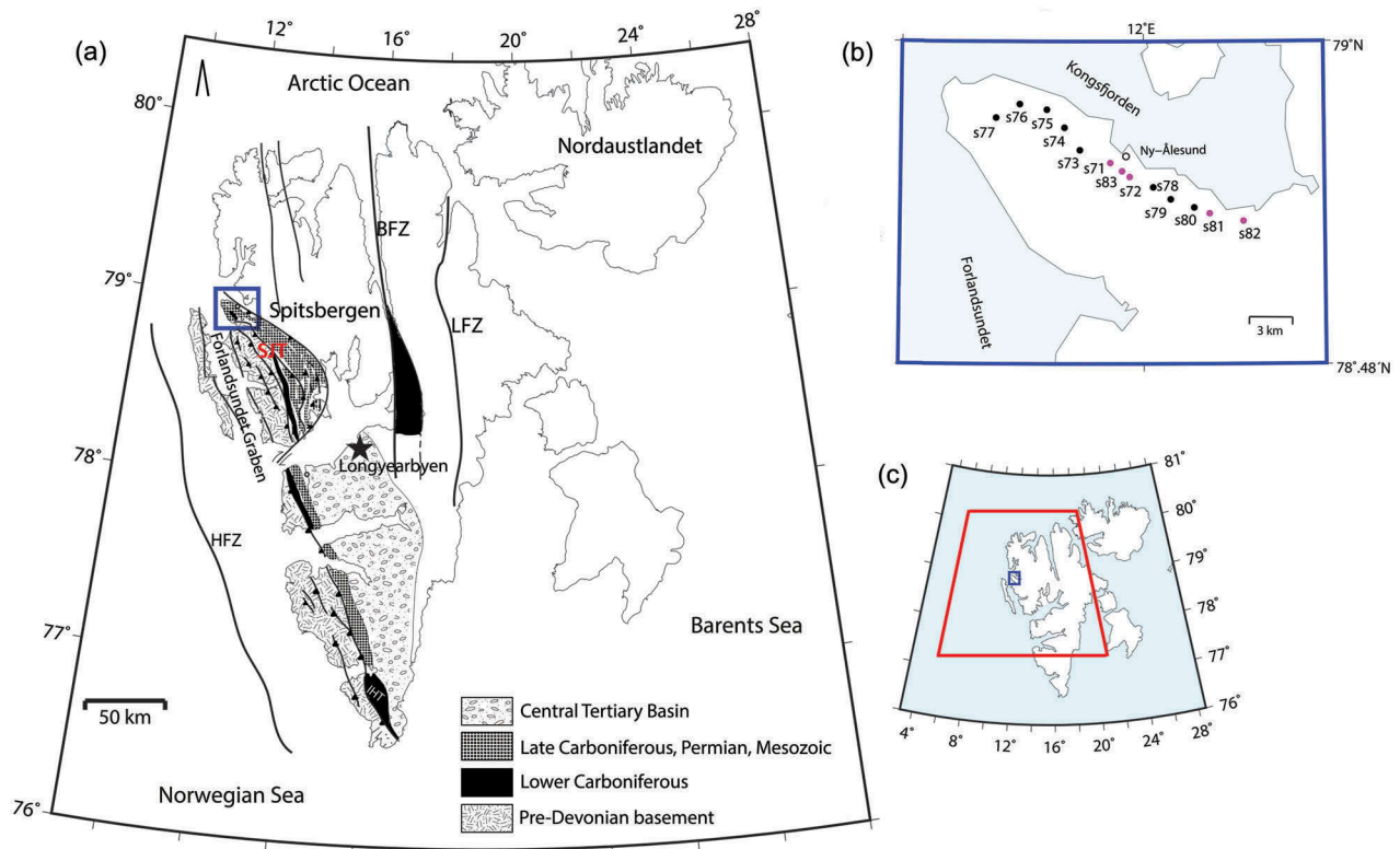
Figure 1. (a) The Svalbard Archipelago with its Tertiary affected section along the transform Hornsund Fault Zone (HFZ) highlighted. The map includes locations of Carboniferous basin strata: the Billefjorden Trough adjacent to the Billefjorden Fault Zone (BFZ), the Lomfjorden Fault zone (LFZ), Inner Hornsund Trough (IHT) and St. Jonsfjorden Trough (SJT). Note also the Tertiary Forlandsundet Graben just south of Brøggerhalvøya. The map is modified and redrawn from Bergh et al. (2000) and Saalman & Thiedig (2002). (b) The MT studied area on Brøggerhalvøya, also represented in (a) and (c) with blue frames. The MT sites are indicated by the black dots and the pink dots denote sites with measured vertical magnetic fields in addition to the horizontal EM components. (c) The red box indicates the surface area of our 3D model.
