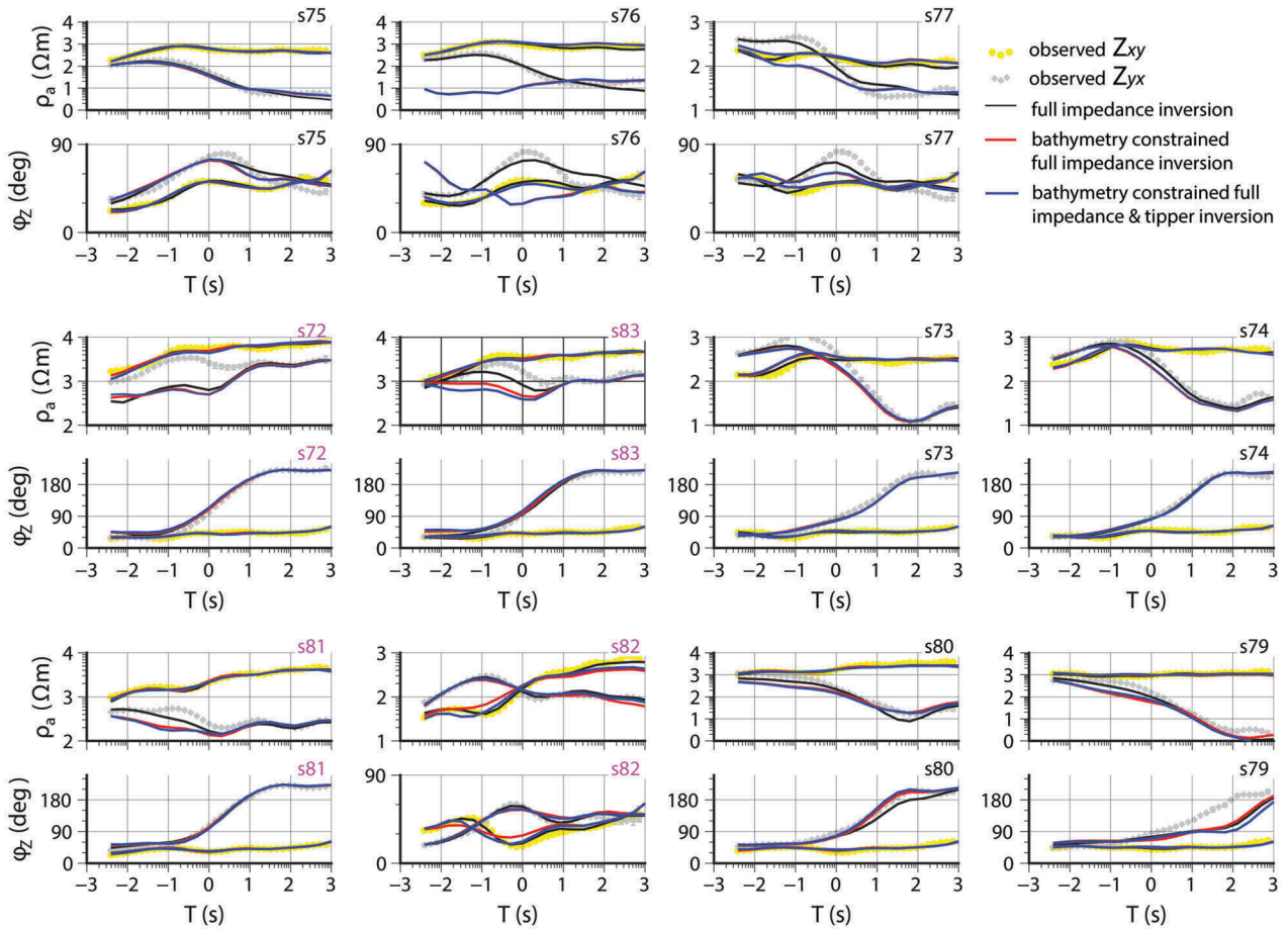
Figure 8. Data misfit between the observed data and results of three different 3D inversion procedures. The misfit is presented site by site for the observed Z_{xy} (yellow dots) and Z_{yx} (grey dots) impedance components in measurement coordinate system. The site names in purple represent the sites with the tipper data included in the inversion. For each site the apparent resistivity ( \Omega\text{m} ) and the phase (deg) parameters are presented in the top and bottom panels, respectively. The data fit for the model presented in Fig. 6 (full impedance inversion; \text{RMS} = 1.68 ) is denoted with black solid lines, when bathymetry is included in the modelling ( \text{RMS} = 2.17 ) in red solid lines and the final model (Fig. 7a, \text{RMS} = 2.2 ) data fits are shown with blue solid lines. The sites are ordered from top left to bottom right matching the MT profile's WNW–ESE direction and in the same order as in Fig. 4.
