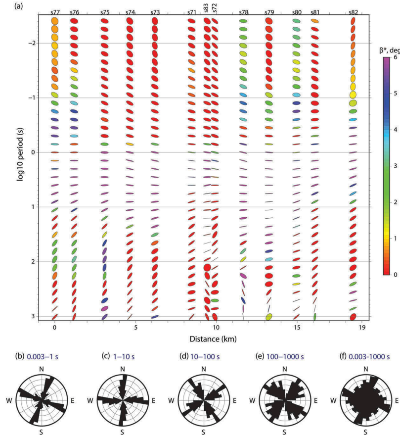
Figure 2. Geoelectric strike and dimensionality. (a) Phase tensor ellipses of the 13 measured sites with their error accounted skew angles ( \beta^* ) in colour fills. (b – e) Phase tensor strike estimates for period intervals manifesting a collective dimensionality behaviour. (f) Phase tensor strike estimate for the entire data set (0.003–1000 s). The analysis in general indicates strong 3D effects, with some localized underlying 2D structures and a weak regionally dominant strike direction suitable for the entire data set.
