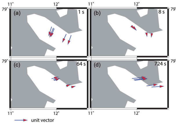
Figure 3. Real part of the induction arrows of the sites s71, s83, s72, s81 and s82 respectively in north-west-south-east direction, in Wiese convention. The arrows are plotted for 1, 8, 64 and 724 seconds in (a) through (d), respectively. The strike directions indicated by the arrows display a reasonable match with the phase tensor strike estimates shown in Fig. 2b–e.
