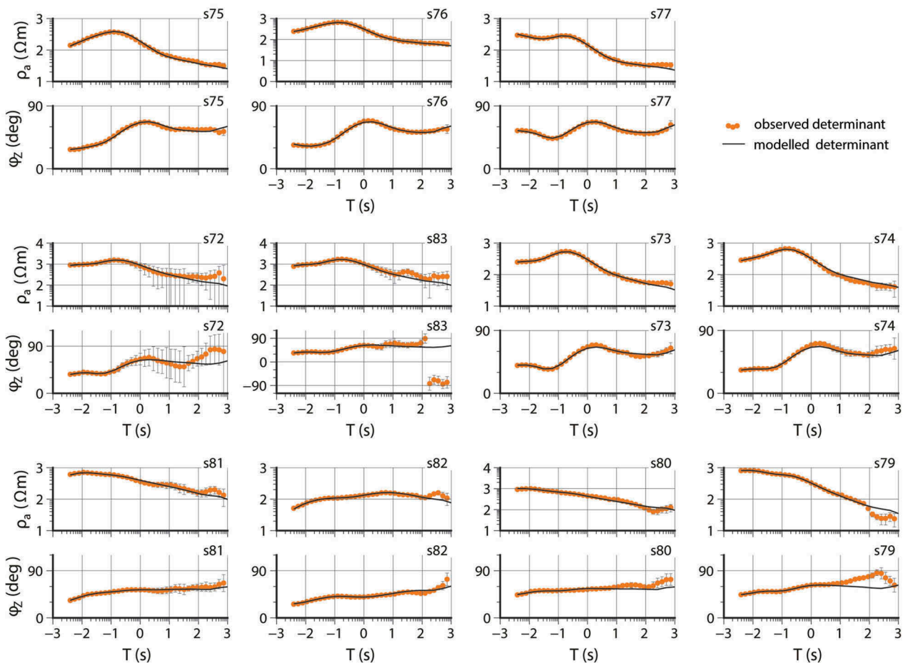
Figure 4. The site by site data misfit between the observed (orange dots) and predicted (black solid lines) determinant data apparent resistivity ( \Omega\text{m} in log10 scale) and phase (deg) parameters underlying the preferred 2D inversion model displayed in Fig. 5b having 1.16 as its overall RMS misfit. All the modelled sites are included in the plot ordered from top – bottom right following the MT profile's WNW–ESE direction. The y axes are given in log10 scales in seconds.
