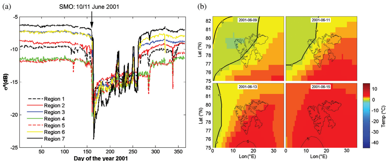
Fig. 8 Synchronous melt onset over all of Svalbard: (a) \sigma_{mean}^o -time series for seven Svalbard regions in 2001, and (b) US National Centers for Environmental Prediction and US National Center for Atmospheric Research (NCEP/NCAR) maps of air-temperature fields from 9 to 15 June 2001.
