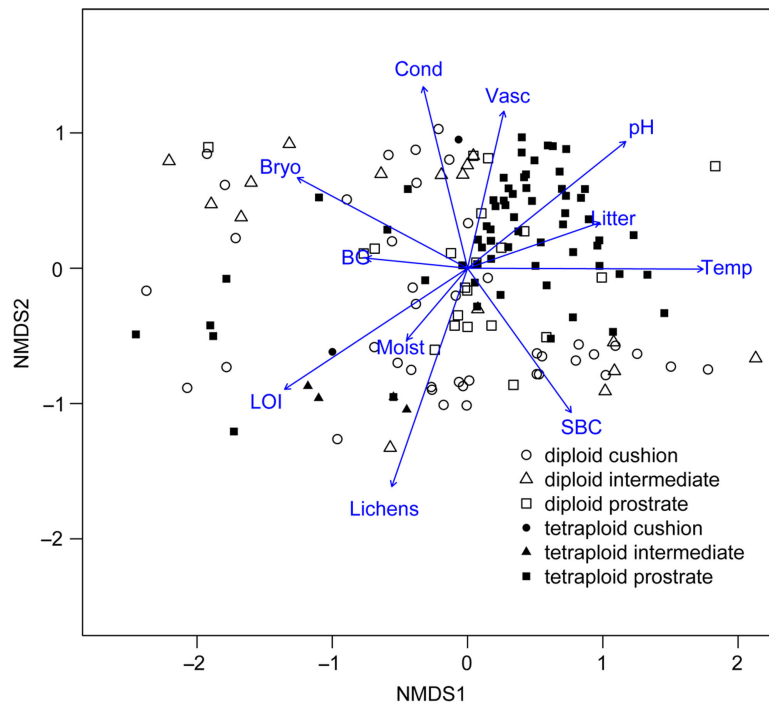
Fig. 3 Non-metric multidimensional scaling (N-MDS) plot showing 148 vegetation plots where diploid and tetraploid individuals of Saxifraga oppositifolia were sampled in Svalbard, including 11 fitted environmental variables. Plots with triploids, plots without vascular vegetation cover and plots from two sampling sites in Wijdefjorden (Location 5; Table 1), which had a strongly deviating species composition compared to the other sampling sites, were excluded from the presented multivariate analysis, in order to achieve a better resolution of the remaining sites. The following terms have been abbreviated: bare ground (BG), bryophyte cover (Bryo), conductivity (Cond), lichen cover (Lichens), coverage of litter (Litter), loss on ignition (LOI), soil moisture (Moist), soil pH (pH), soil biological crust (SBC), soil temperature (Temp) and vascular plant cover (Vasc).
