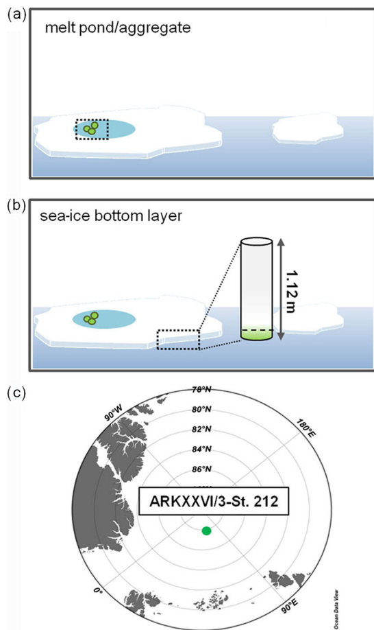
Fig. 1 (a) Melt-pond aggregate and (b) sea-ice bottom layer (sea-ice–water interface; 10 cm) habitats. (c) The position of sampling station 212 in the Arctic Ocean (ARKXXVI/3 cruise).
