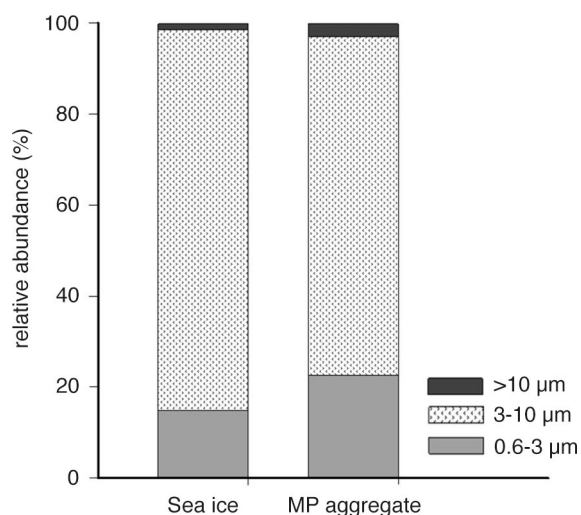
Fig. 2 Histogram of the protist cell size distribution in the sea-ice bottom layer and melt-pond aggregate obtained by flow cytometry.
