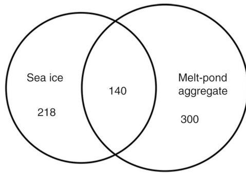
Fig. 3 Venn diagram of the operational taxonomic unit (OTU) overlap between the sea-ice bottom layer and melt-pond aggregate habitats. OTUs were generated with a threshold of 97% identity.
