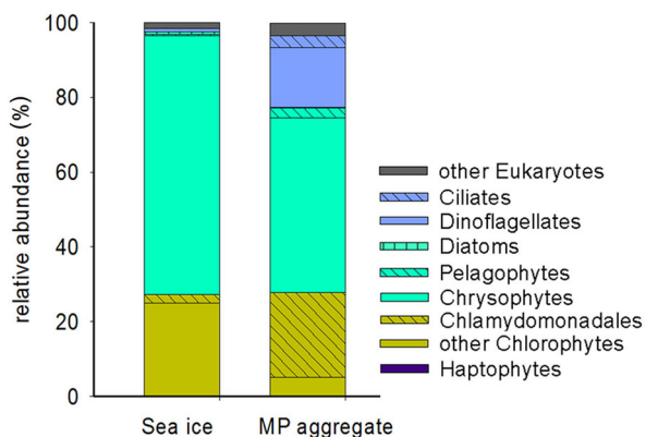
Fig. 4 Histogram showing the relative abundances (%) of major taxonomic groups, obtained by 454-pyrosequencing read distribution in the sea-ice bottom layer and melt-pond aggregate.
