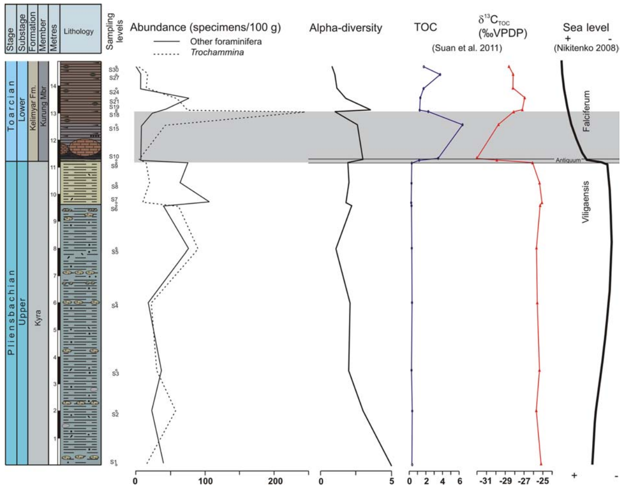
Fig. 7 Abundance of Trochammina vs. rest of foraminifera compared with \alpha -diversity index, as well as the total organic carbon (TOC) and \delta^{13}C from organic matter of Suan et al. (2011), and sea-level fluctuations according to Nikitenko (2008).
