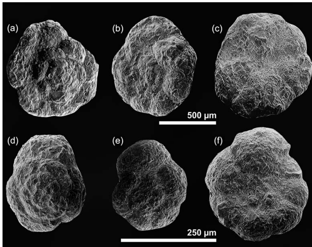
Fig. 3 Scanning electron images of (a, b, c) Trochammina lapidosa , Upper Pliensbachian, microsphaeric form, (a) dorsal view, (b, c) megalosphaeric form, (b) dorsal view, (c) ventral view and (d, e, f) Trochammina kisselmani , Lower Toarcian, (d, f) microsphaeric form, (d) dorsal view, (f) ventral view, megalosphaeric form, (e) dorsal view.
