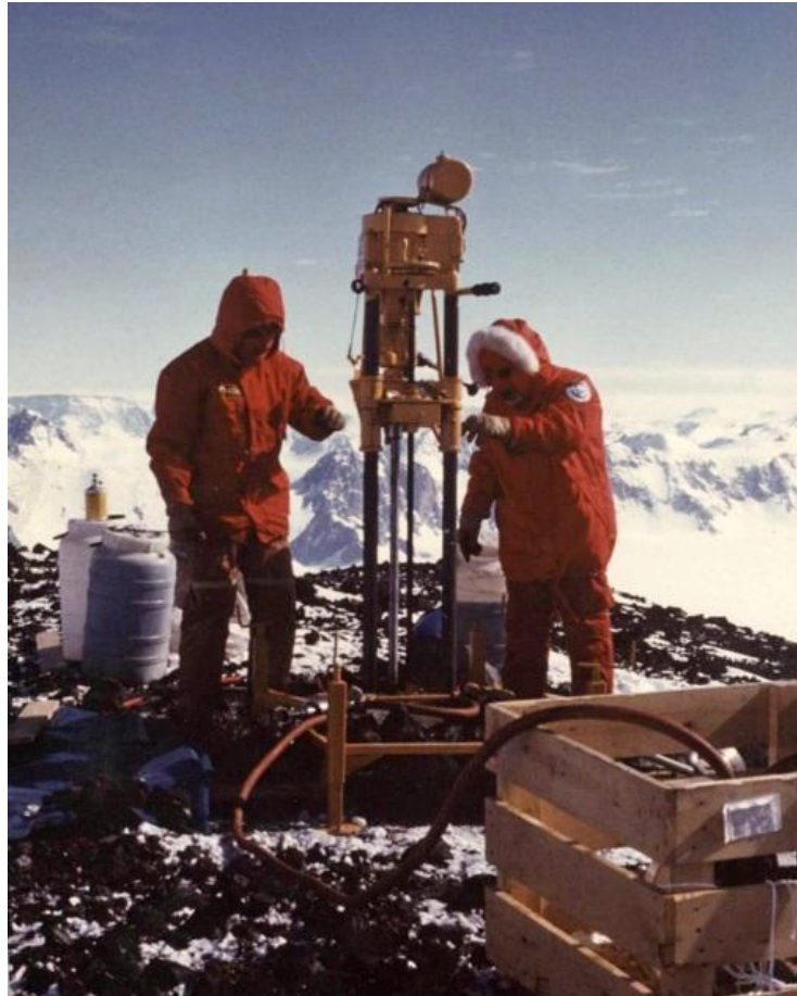
Supplementary Fig. S1. Photograph of the drilling phase for the installation of the tiltmeter at VIL1 station.
