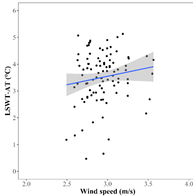
Supplementary Fig. S1. The relationship between the difference between lake surface water temperature (LSWT) and air temperature (AT) and wind speed in summer. The grey shading represents the confidence interval based on 95% confidence level.
